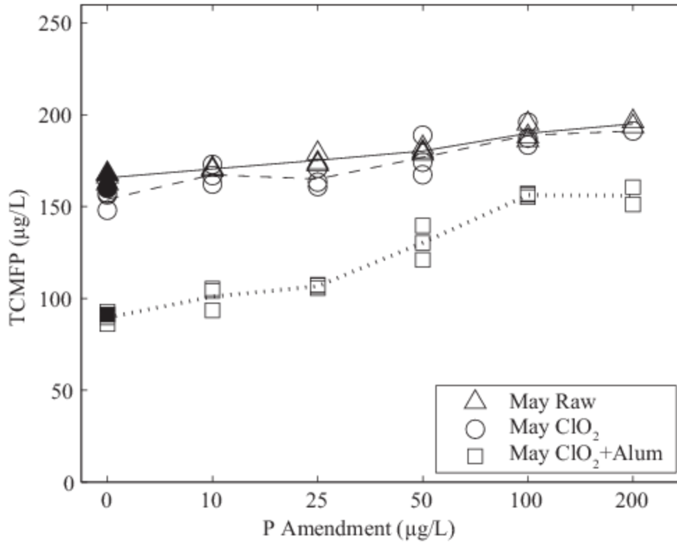
Figure 7 – Trichloromethane formation potential (TCMFP) as a function of phosphorus (P) amendment for May 30 raw and treated waters ( \text{ClO}_2 dose of 1 \text{ mg L}^{-1} as \text{Cl}_2 and alum dose of 40 \text{ mg L}^{-1} ). The N dose for all P-amended samples was 2,000 \text{ } \mu\text{g L}^{-1} . Lines represent triplicate averages; filled markers represent blank samples without any nutrient amendment.
